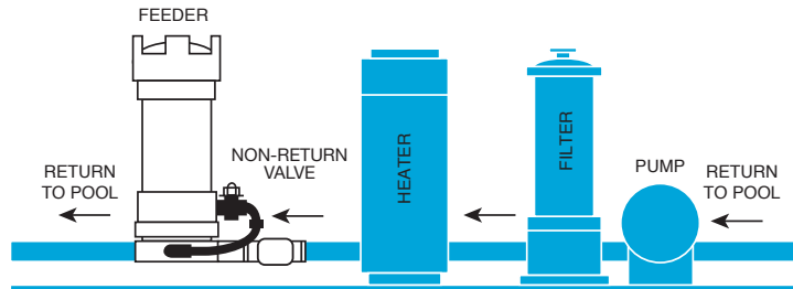
Illustration of model 320 Feeder
