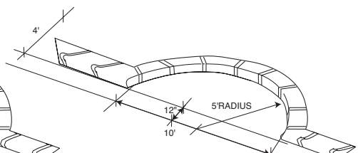
10FT LOW PROFILE ROMAN END
