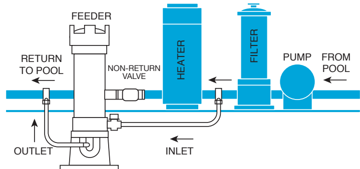
Illustration of model 300 Feeder
