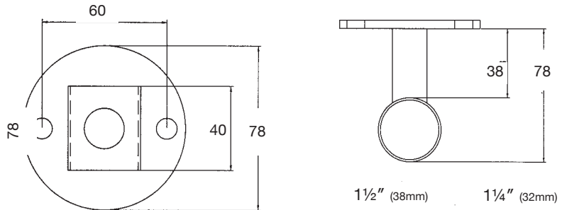
Dimensions for stainless steel 1.25" (32mm) Handrail Bracket
