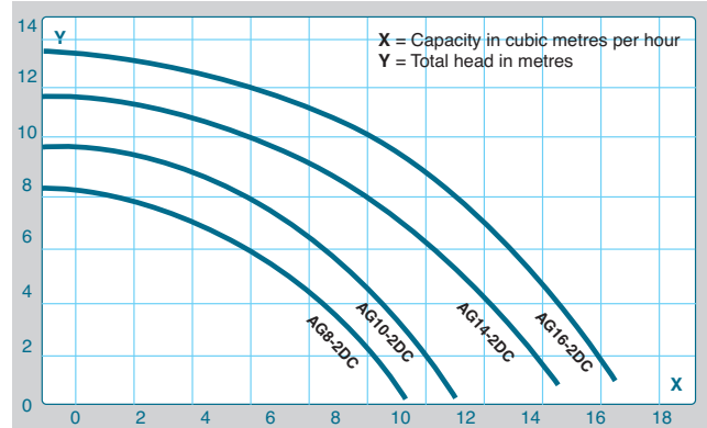
Performance Curve
