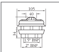
Fixed Grate with Back Nut – HD54PLT/5
