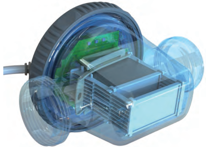
Solid titanium plates with ruthenium treatment
