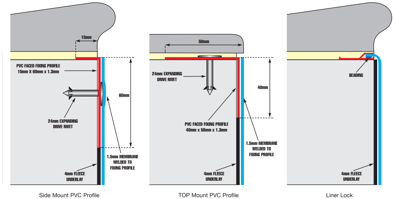
Side Mount PVC Profile
