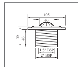
Fixed Grate – HD54C/5
