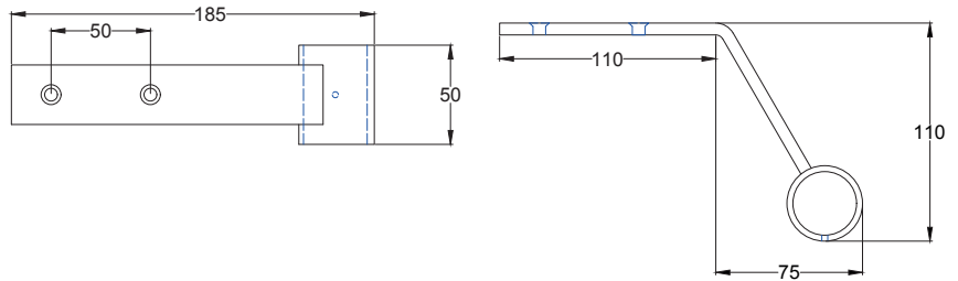
Dimensions for stainless steel 1.25" (32mm) Handrail Bracket
