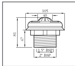
Fixed Grate – HD54LT/5
