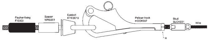
Towing End - Width Fixing
